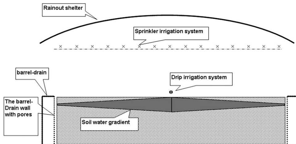
Fig. 1. A sketch map of the DR screening facility. The water stress was conducted at the reproductive stage. Sprinkler irrigation was ceased and the water in the barrel-drain was drained out until the water level was below the water table. Therefore, soil water led into the barrel-drain through pores in the barrel-drain wall. Drip irrigation was initiated to maintain the soil water in the middle of the field. As a result, the water gradient within the test field was established.
